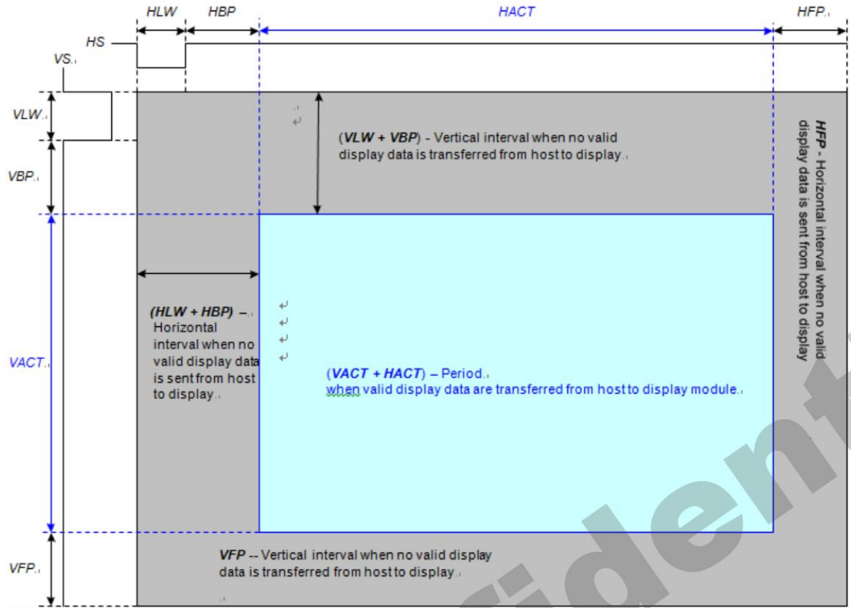
General timing diagram
