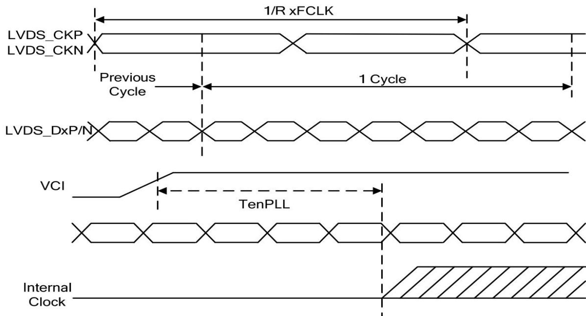
Figure LVDS figure
