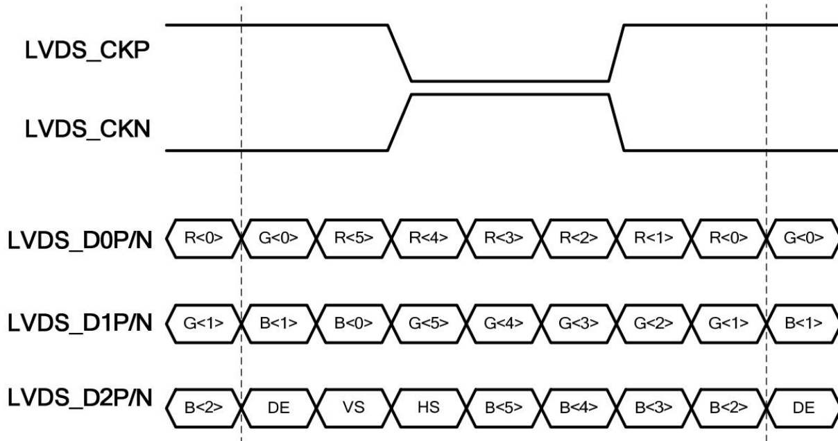
6-bit LVDS input_VESA format
