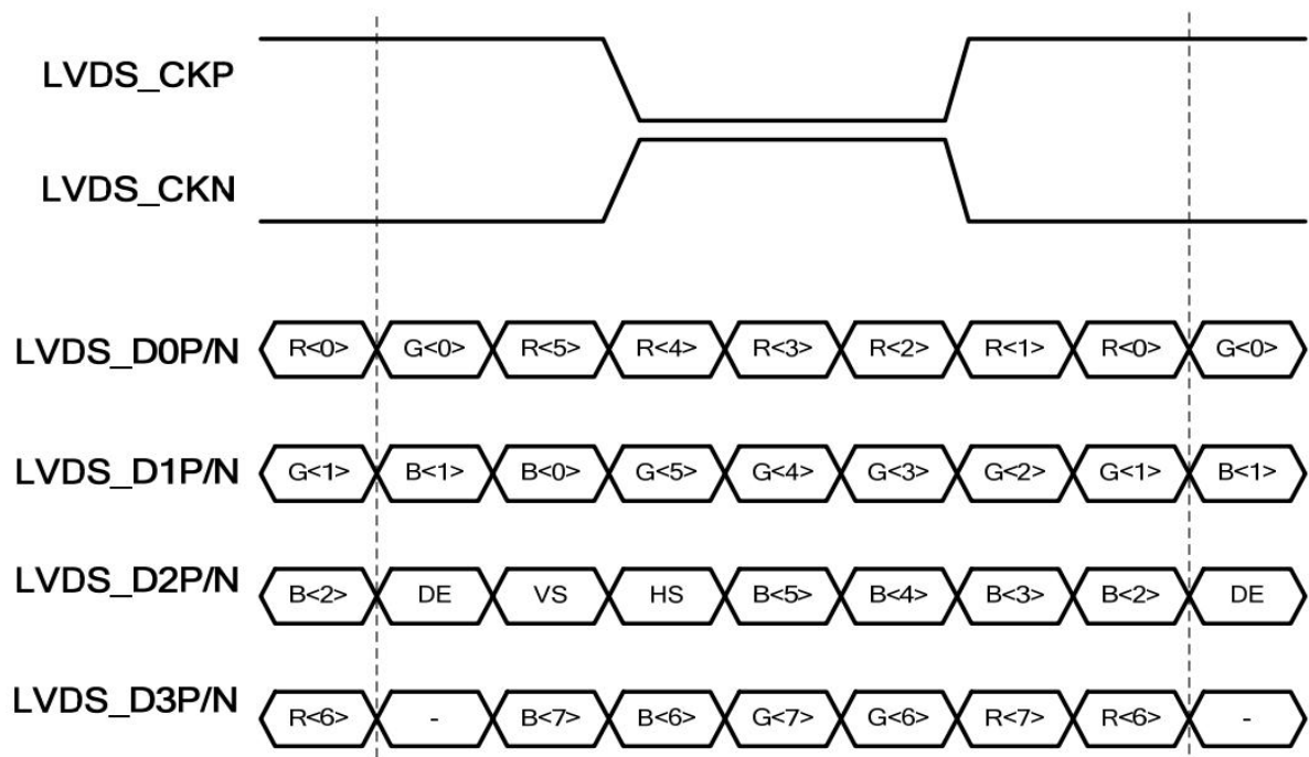
8-bit LVDS input_VESA format
