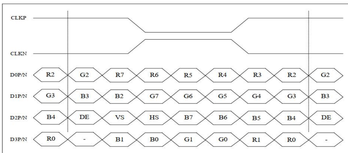
8-bit RGB LVDS JEIDA input timing
