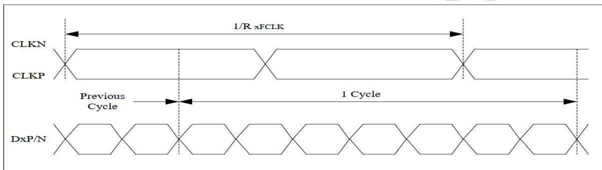
LVDS mode AC electrical characteristics
