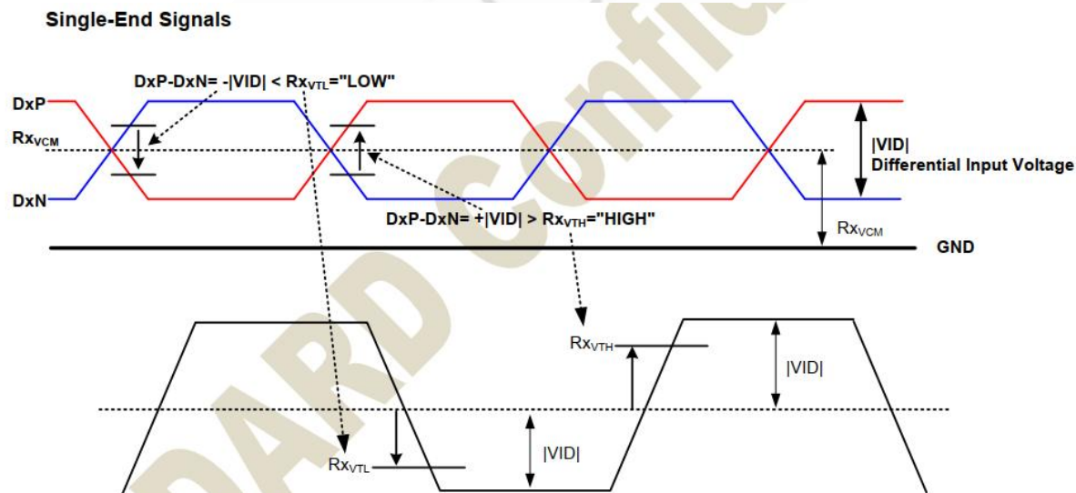
Figure 11.1: LVDS input timings
