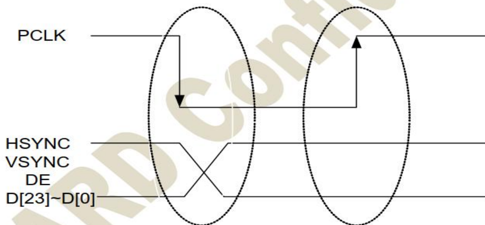
Figure 7.9: PCLK cycle
