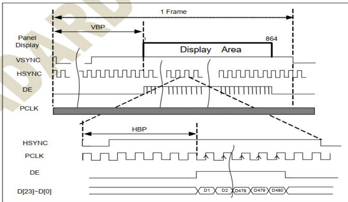
Figure 7.8: RGB (800RGB x 480) timing diagram
