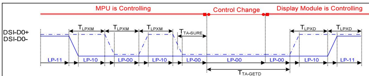
Bus Turn-around Procedure
